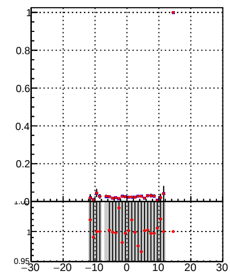
Fake rate vs d —•— DQM_TT_mkFit-DQM_lowptq_orig —•— DQM_TT_mkFit-DQM_lowptq_mod12
