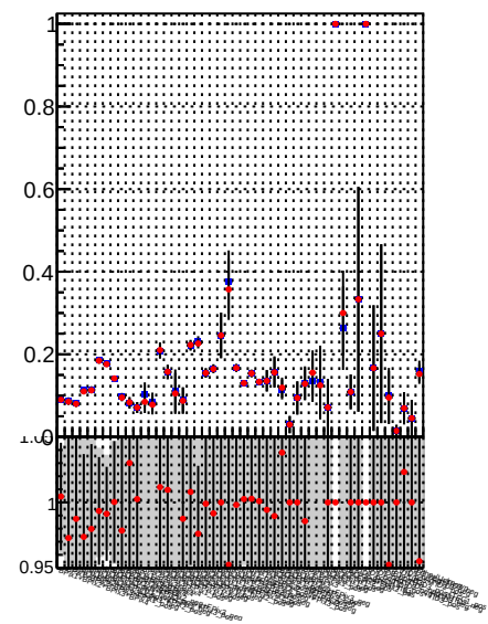
Fake rate vs. —•— DQM TT mkFit-DQM_lowptq_orig —•— DQM TT mkFit-DQM_lowptq_mod12
