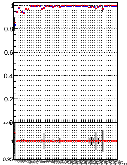
Fake rate vs. DQM_TT_mkFit-DQM_lowptq_orig DQM_TT_mkFit-DQM_lowptq_modi2
