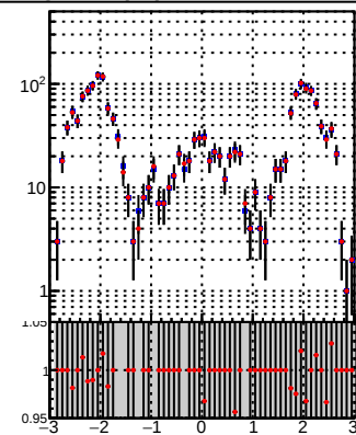
—•— DQM_TT_mkFit-DQM_lowptq_orig —•— DQM_TT_mkFit-DQM_lowptq_modi2
