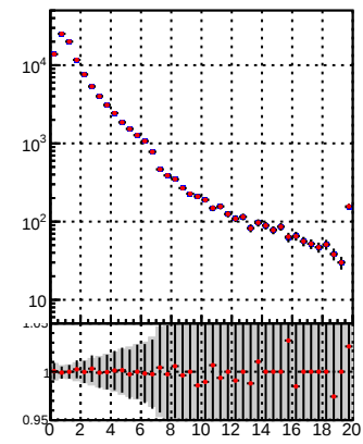
N of reco track vs. \chi^2 —●— DQM_TT mkFit-DQM_lowptq_orig —●— DQM_TT mkFit-DQM_lowptq_modi2
