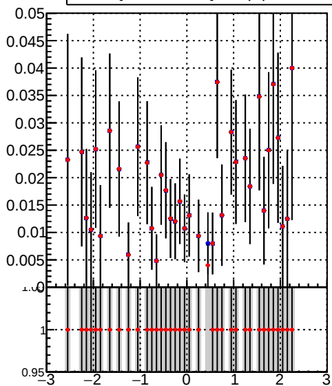
—•— DQM_TT_mkFit-DQM_lowptq_orig —•— DQM_TT_mkFit-DQM_lowptq_modi2
