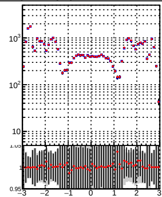
DQM_TT_mkFit-DQM_lowptq_orig DQM_TT_mkFit-DQM_lowptq_modi2
