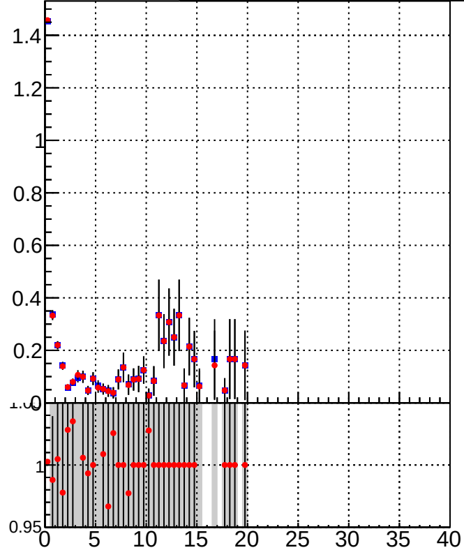
K_S^0 tracking fake rate vs p_T (Detailed View) Legend: \text{DQM\_TT\_mkFit-DQM\_lowptq\_orig} (Blue squares) \text{DQM\_TT\_mkFit-DQM\_lowptq\_modi2} (Red circles)
