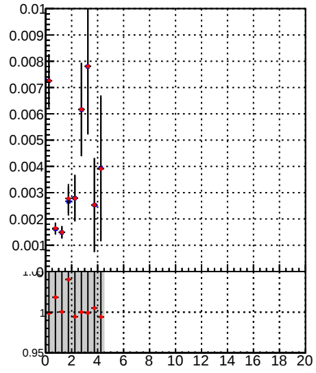
Fake rate vs. — DQM TT mkFit-DQM_lowptq_orig — DQM TT mkFit-DQM_lowptq_mod12
