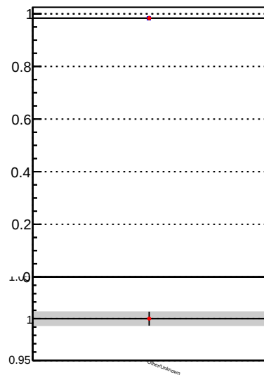
Fake rate vs. —•— DQM_TT_mkFit-DQM_lowptq_orig —•— DQM_TT_mkFit-DQM_lowptq_modi2
