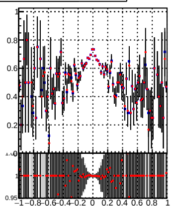
DQM_TT_mkFit-DQM_lowptq_modi2
