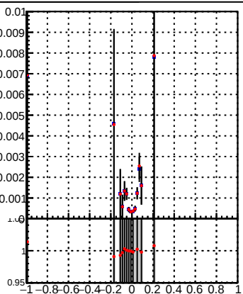
DQM_TT_mkFit-DQM_lowptq_orig
