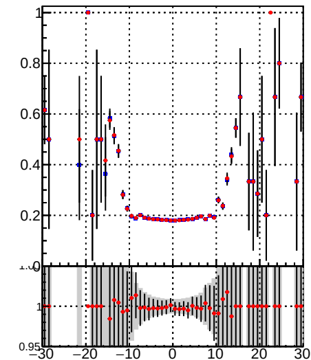
—•— DQM_TT_mkFit-DQM_lowptq_orig —•— DQM_TT_mkFit-DQM_lowptq_modi2
