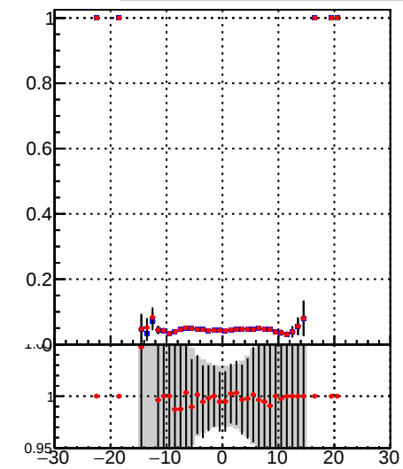
—■— DQM_TT_mkFit-DQM_lowptq_orig —■— DQM_TT_mkFit-DQM_lowptq_modi2
