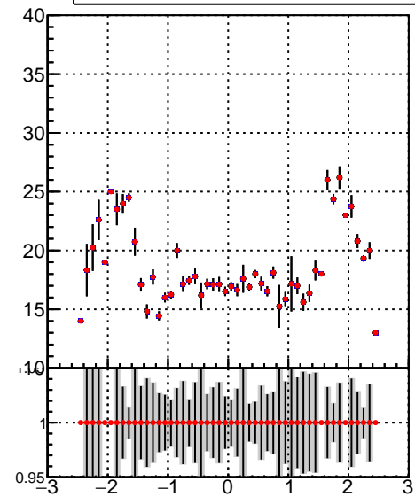
DQM_TT_mkFit-DQM_lowptq_modi2
