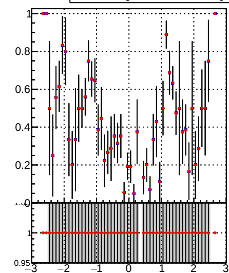
■ DQM_TT_mkFit-DQM_lowptq_orig ● DQM_TT_mkFit-DQM_lowptq_modi2
