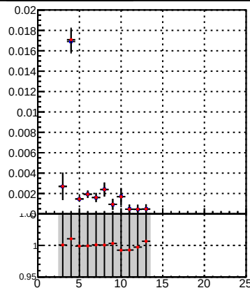
Legend: DQM_TT_mkFit-DQM_lowptq_orig (blue line with circles), DQM_TT_mkFit-DQM_lowptq_modi2 (red line with crosses)
