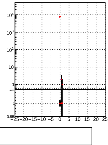
N of associated tracks (simToReco) vs dxy(PV)
