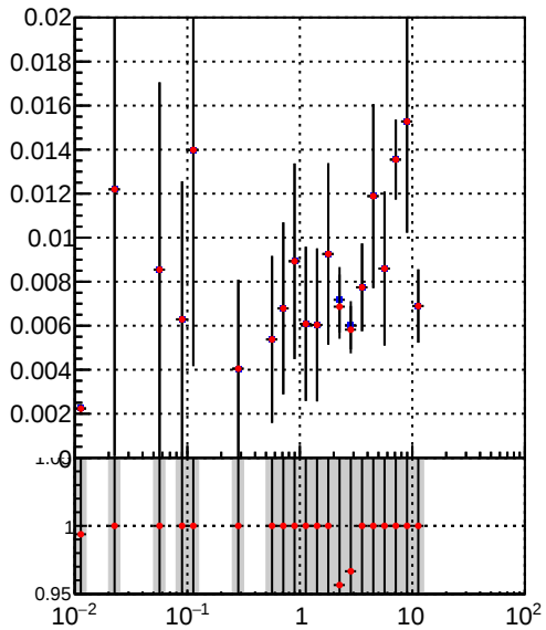
Efficiency vs vertpos Legend: DQM_TT_mkFit-DQM_lowptq_orig DQM_TT_mkFit-DQM_lowptq_modi
