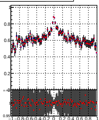
DQM_TT_mkFit-DQM_lowptq_modi
