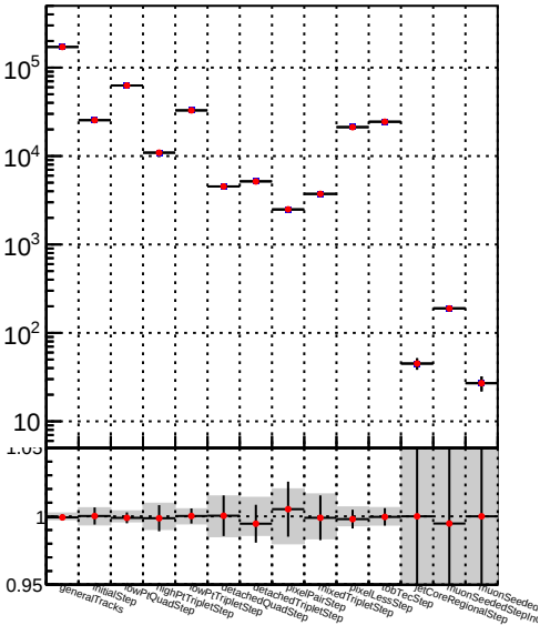
Number —●— DQM_TT__mkFit-DQM_lowptq_modi
