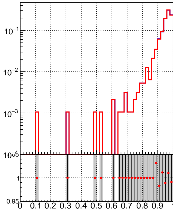
RecoPVAssoc2GenPVMatched_Purity
