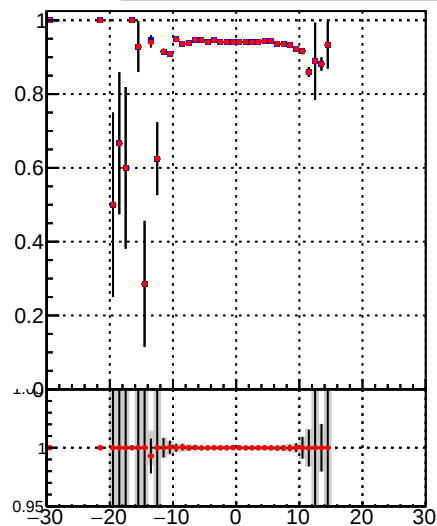
—•— DQM_TT_mkFit-DQM_lowptq_orig —•— DQM_TT_mkFit-DQM_lowptq_modi
