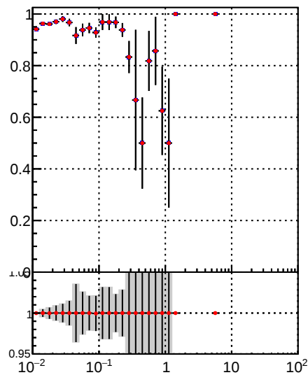
—•— DQM_TT_mkFit-DQM_lowptq_orig —•— DQM_TT_mkFit-DQM_lowptq_modi
