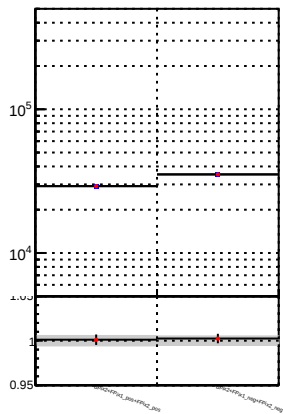
N of reco track vs. \chi^2 for different \chi^2 bins
