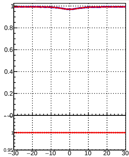
DQM_TT_mkFit-DQM_lowptq_orig DQM_TT_mkFit-DQM_lowptq_modi
