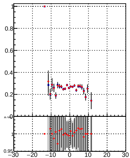
Fake rate vs d Legend: Blue line with dots: DQM TT mkFit-DQM_lowptq_orig Red line with dots: DQM TT mkFit-DQM_lowptq_modi
