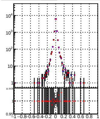
Legend: DQM_TT_mkFit-DQM_lowptq_orig (Black line with grey shaded area) DQM_TT_mkFit-DQM_lowptq_modi (Red line with red shaded area)
