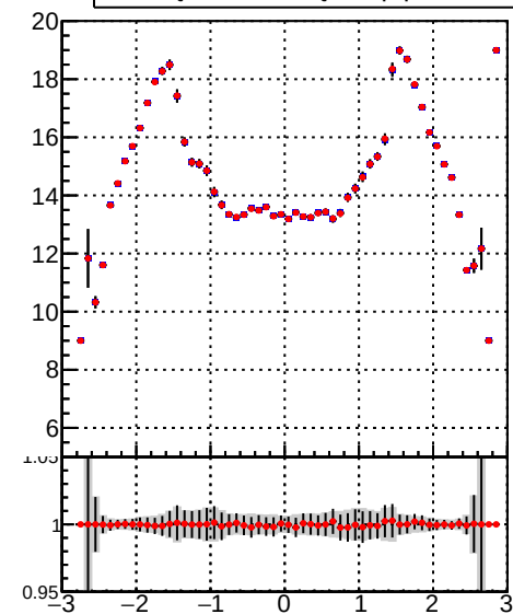
— DQM_TT_mkFit-DQM_lowptq_orig — DQM_TT_mkFit-DQM_lowptq_modi
