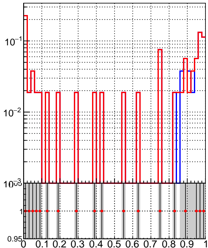
RecoPVAssoc2GenPVNotMatched_Purity
