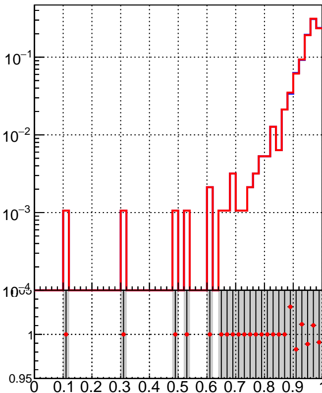
RecoPVAssoc2GenPVMatched_Purity
