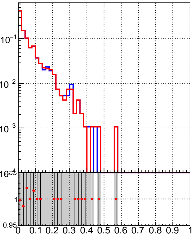
RecoPVAssoc2GenPVMatched_missing
