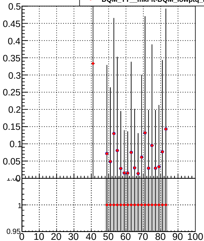
■ DQM_TT_mkFit-DQM_lowptq_orig ● DQM_TT_mkFit-DQM_lowptq_modi
