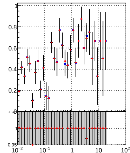
—•— DQM_TT_mkFit-DQM_lowptq_orig —•— DQM_TT_mkFit-DQM_lowptq_modi
