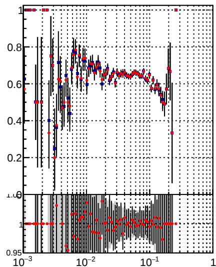
■ DQM_TT_mkFit-DQM_lowptq_orig ■ DQM_TT_mkFit-DQM_lowptq_modi
