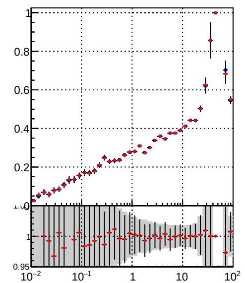
Legend: DQM_TT_mkFit-DQM_lowptq_orig DQM_TT_mkFit-DQM_lowptq_modi
