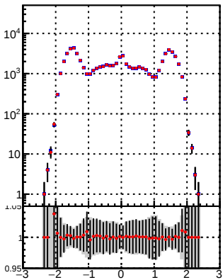
N of reco track vs \eta —•— DQM_TT_mkFit-DQM_lowptq_orig —•— DQM_TT_mkFit-DQM_lowptq_modi
