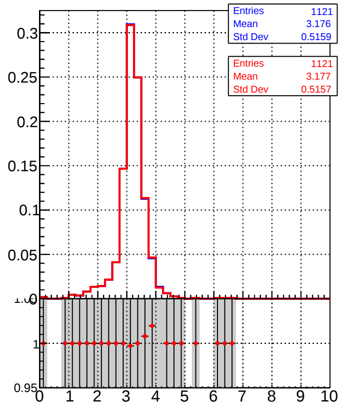
Legend: DQM_TT_mkFit-DQM_lowptq_orig DQM_TT_mkFit-DQM_lowptq_modi
