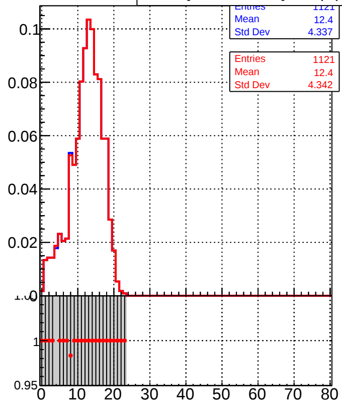
Legend: DQM_TT_mkFit-DQM_lowptq_orig DQM_TT_mkFit-DQM_lowptq_modi
