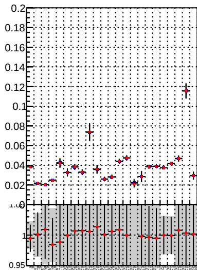
Fake rate vs. DQM TT mkFit-DQM_lowptq_orig DQM TT mkFit-DQM_lowptq_modi
