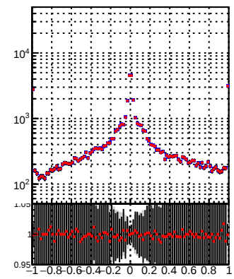
Legend: DQM_TT_mkFit-DQM_lowptq_orig (Blue line with dots) DQM_TT_mkFit-DQM_lowptq_modi (Red line with dots)
