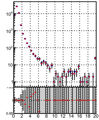
Legend: - Blue line with dots: DQM TT mkFit-DQM_lowptq_orig - Red line with dots: DQM TT mkFit-DQM_lowptq_modi - Grey shaded area: verSet
