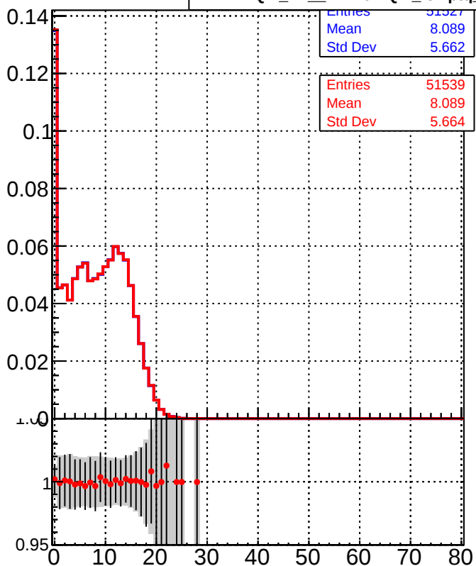
— DQM_TT_mkFit-DQM_lowptq_orig — DQM_TT_mkFit-DQM_lowptq_modi
