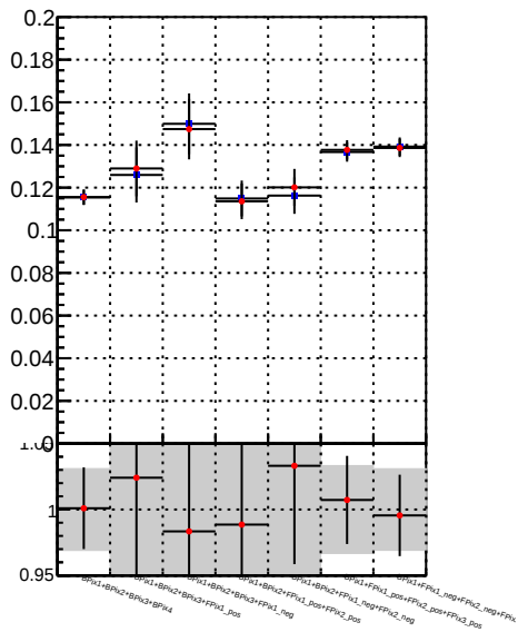
Fake rate vs. —•— DQM_TT_mkFit-DQM_lowptq_orig —•— DQM_TT_mkFit-DQM_lowptq_modi
