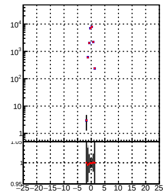
Legend: DQM_TT_mkFit-DQM_lowptq_orig (black histogram) DQM_TT_mkFit-DQM_lowptq_modi (red line with markers)
