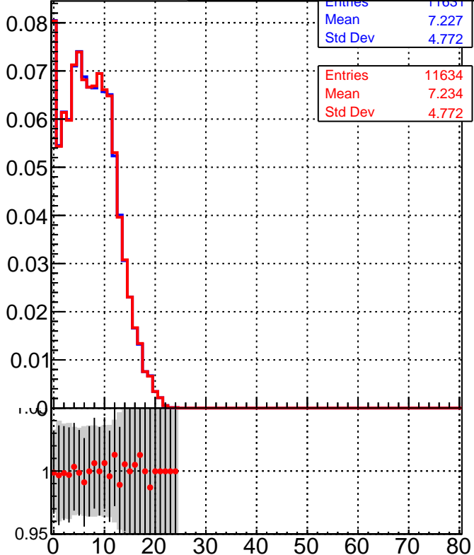
■ DQM_TT_mkFit-DQM_lowptq_orig ● DQM_TT_mkFit-DQM_lowptq_modi
