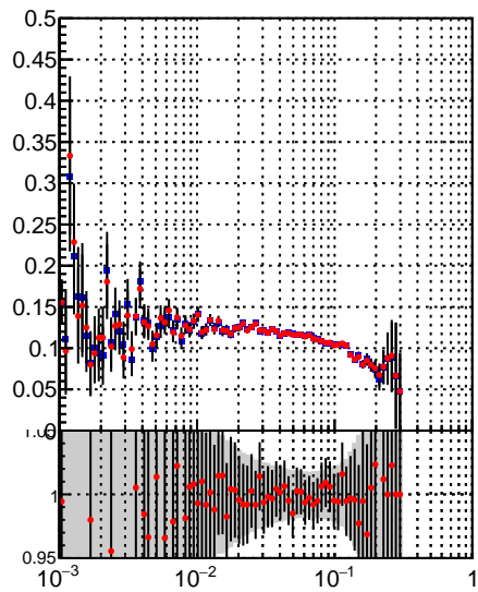
—●— DQM_TT_mkFit-DQM_lowptq_orig —●— DQM_TT_mkFit-DQM_lowptq_modi
