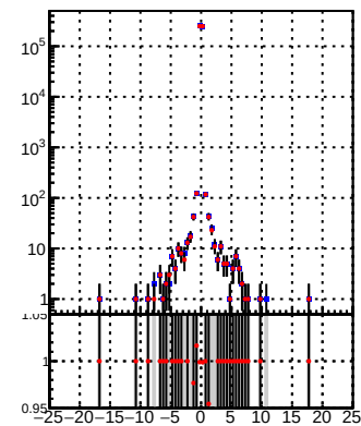
Legend: —•— DQM_TT_mkFit-DQM_lowptq_orig —•— DQM_TT_mkFit-DQM_lowptq_modi
