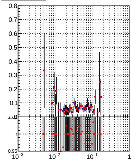
—•— DQM_TT_mkFit-DQM_lowptq_orig —•— DQM_TT_mkFit-DQM_lowptq_modi
