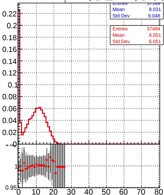
— DQM_TT_mkFit-DQM_lowptq_orig — DQM_TT_mkFit-DQM_lowptq_modi
