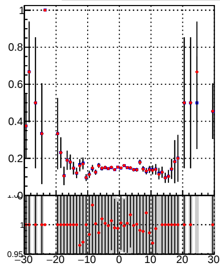
—•— DQM_TT_mkFit-DQM_lowptq_orig —•— DQM_TT_mkFit-DQM_lowptq_modi
