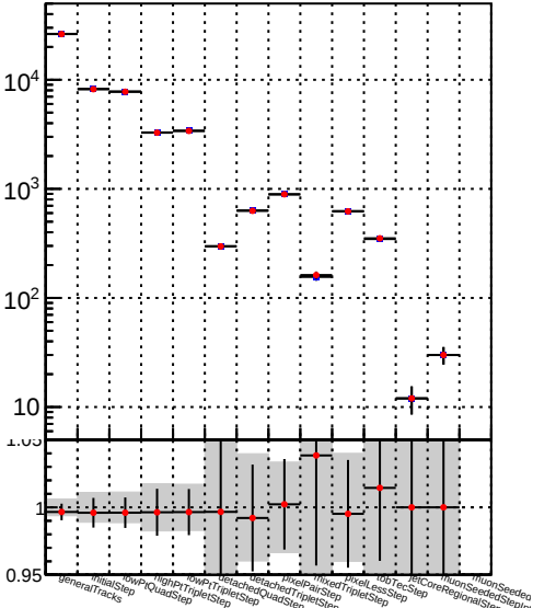
Number —●— DQM_TT__mkFit-DQM_lowptq_modi
