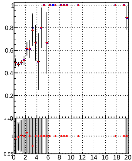
Fake rate vs. — DQM_TT_mkFit-DQM_lowptq_orig — DQM_TT_mkFit-DQM_lowptq_modi
