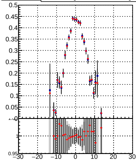
—●— DQM_TT_mkFit-DQM_lowptq_orig —●— DQM_TT_mkFit-DQM_lowptq_modi
