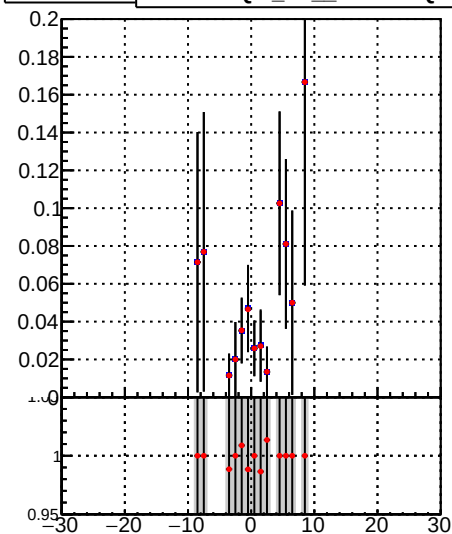
Fake rate vs v Legend: DQM_TT_mkFit-DQM_lowptq_orig (grey bar) DQM_TT_mkFit-DQM_lowptq_modi (red line with markers)
